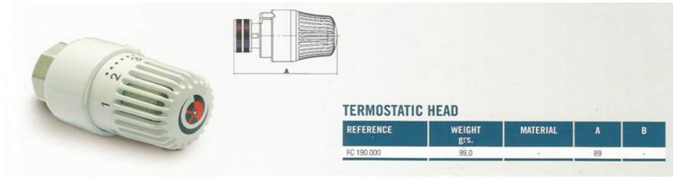
Thermostatic Head
